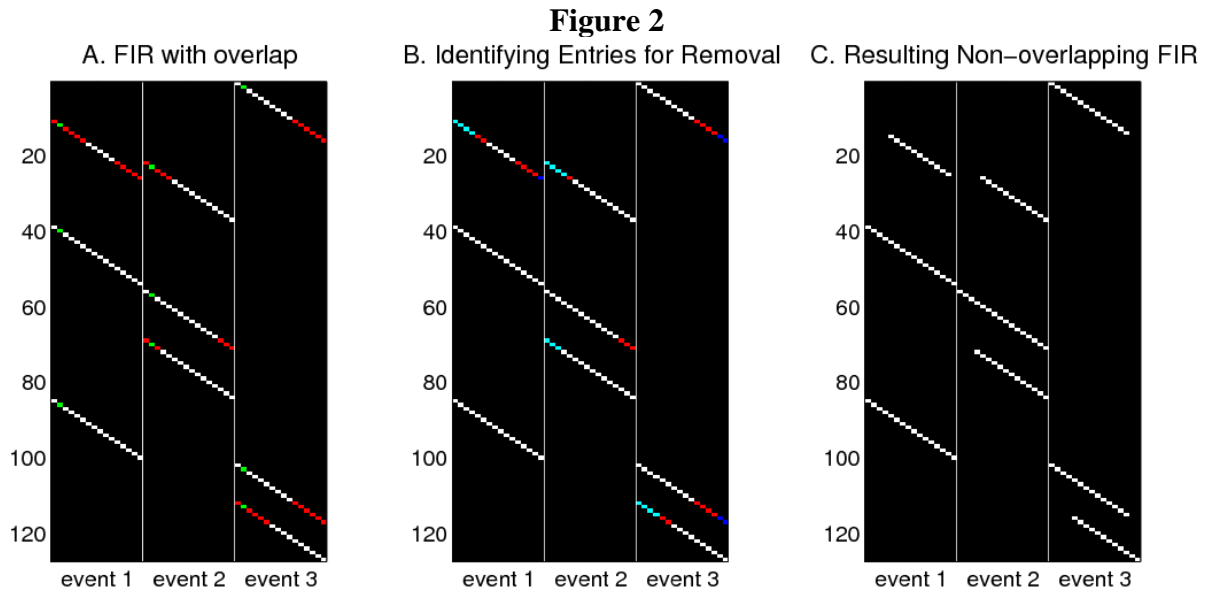
Figure 2. Example for estimating event-related BOLD responses with a Finite Impulse Response (FIR) model. (A) Original FIR design for three different event types with three trials each. The FIR for each event contains as many regressors as specified time bins (16 in this example). The stimulus onset is marked by the green bin. Due to the relatively long time window and the rapid presentation time, some of the bins are overlapping between and within event types (marked in red). Estimating this FIR design would yield parameter estimate for these bins that are not identical to the mean BOLD signal in each bin. (B) rfxplot resolves this ambiguity by removing these entries from the FIR design. Assuming that the most important part of the BOLD response is its peak approximately 4-5 sec after stimulus onset, rfxplot starts removing entries from the beginning of the time window until 2 seconds after stimulus onset (marked in cyan). If this does not completely resolve the overlap, then overlapping entries are removed from the end of the time window (marked in blue). (C) The resulting FIR design after the removal of overlapping bins. This procedure implemented in rfxplot tries to preserve the bin structure with an emphasis on those bins when the maximum BOLD response is expected (~4-5 sec after stimulus onset). However, it also insures that the parameter estimates for the FIR design will always be identical to the average BOLD signal in each bin.
